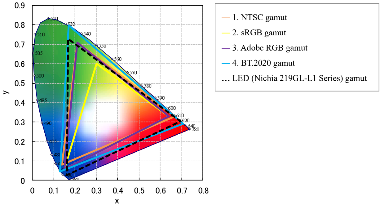
Figure 3. Comparison of the Gamut Ranges of LEDs and Major Color Gamut Specifications
