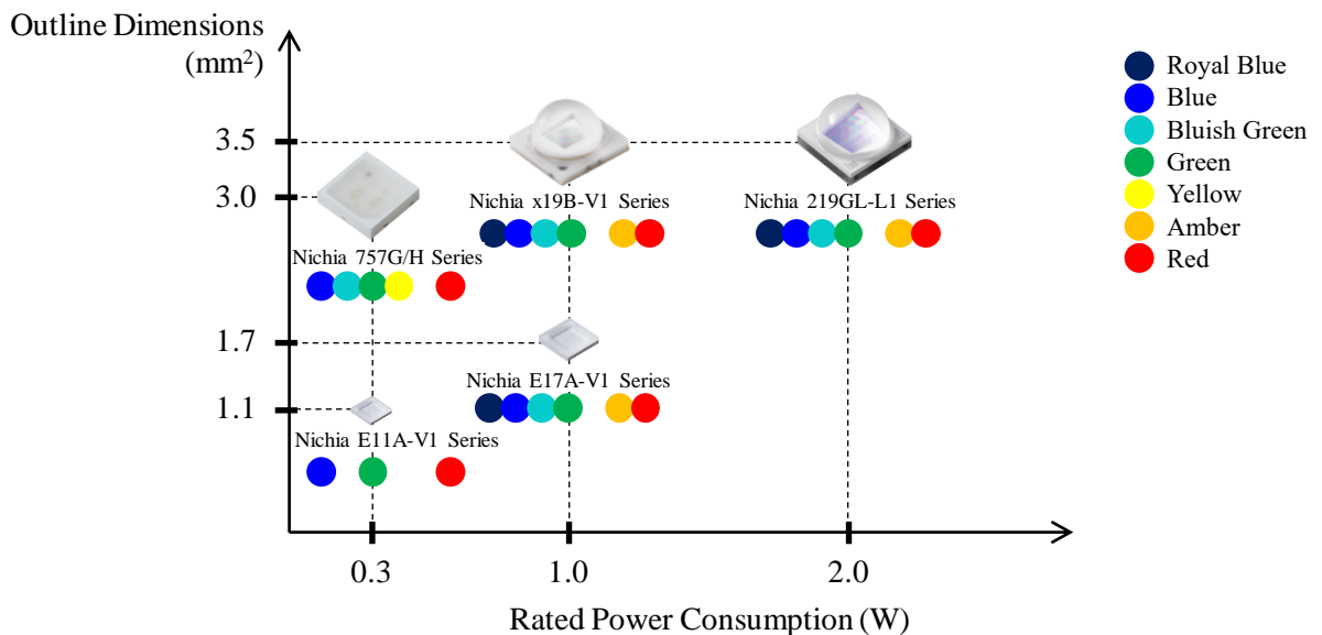
Figure 2. Color Options and Specifications for Nichia's Discrete Color LED Series 4
